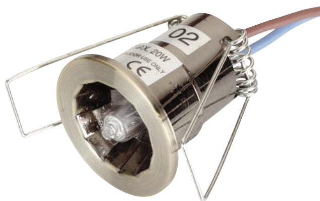
G4 MINIATURE DOWNLIGHTER
