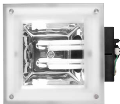
PLC COMPACT FLUORESCENT SQUARE DOWNLIGHTER DROP GLASS
